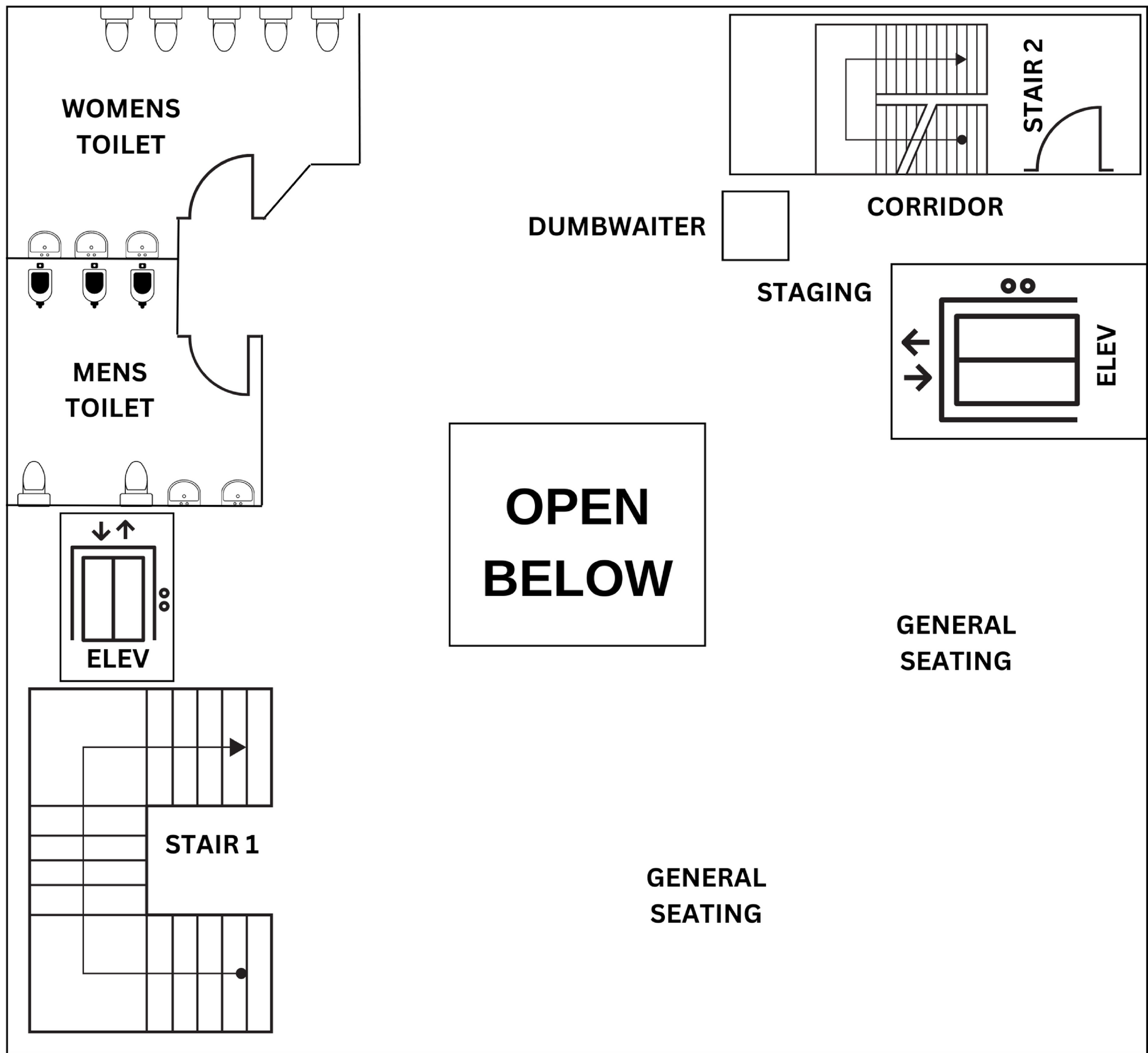
2ND FLOOR
