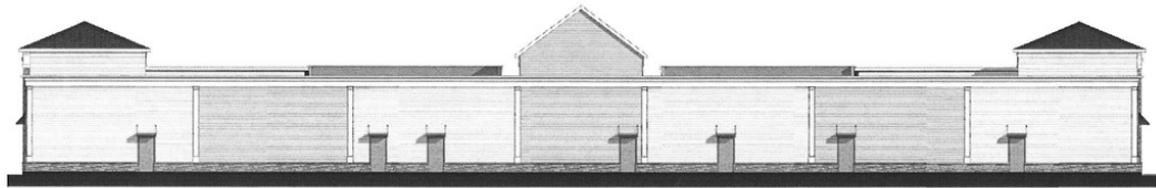
Building Rear Elevation Scale: 1/8" = 1'-0"
